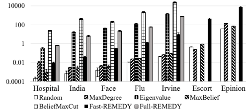
Figure 5: Computation time (y-axis, in seconds) in different contact networks in logarithmic scale.
