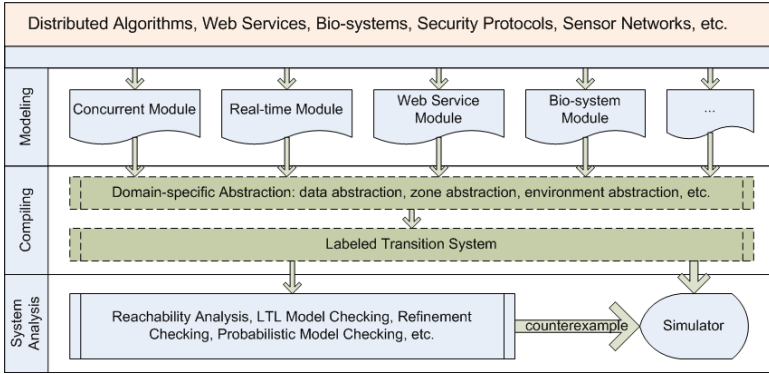
Fig. 1. PAT Architecture
