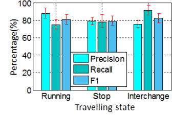
Figure 15: 10-fold cross validation of CRF.
