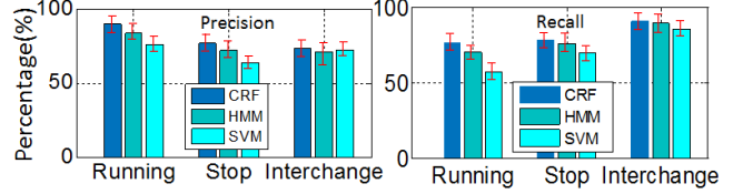
Figure 16: Comparison of inference model.
