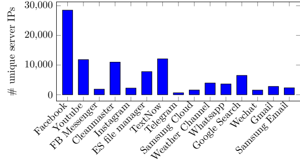
Figure 7: Number of unique server IP addresses for the top 15 apps with most measurement records.
