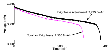
Fig. 32: Battery-aware display.
