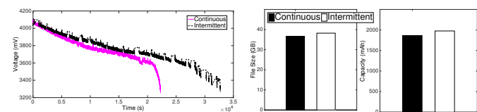
Fig. 2: Continuous vs. intermittent downloading: less consumption does not always lead to longer operation.
