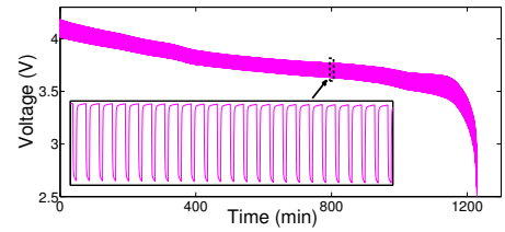
Fig. 8: Discharge a Note 2 battery.
