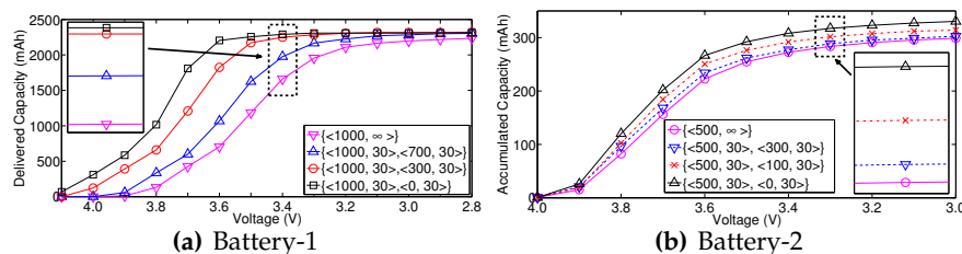
Fig. 31: A larger current gap improves battery capacity delivery further.
