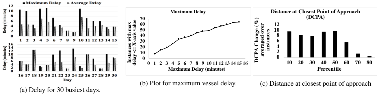
Figure 4: Vessel delay and DCPA plots
