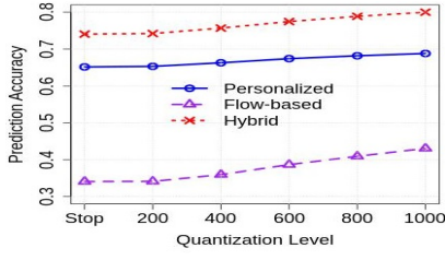
Figure 14: Impact of Spatial Quantization on Prediction Accuracy
