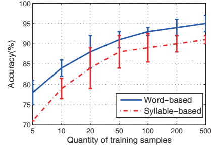
Figure 11: Training overhead.
