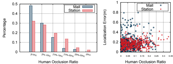
(a) Human Occlusion Distribution (b) Localization Error Figure 19. Human Occlusion Ratio and Impact on Localization
