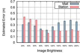
Figure 17. Impact of Illumination
