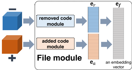
Fig. 2. Architecture of the file module for mapping a file in a given patch to an embedding vector. The input of the module is the removed code and added code of the affected file, denoted by “-” and “+”, respectively.
