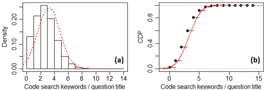
Fig. 11 Collected search query keywords in Stack Overflow– a Keyword frequency PMF b Keyword frequency CDF
