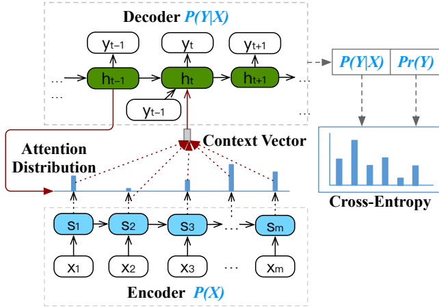
Figure 3: Sequence-to-Sequence model.
