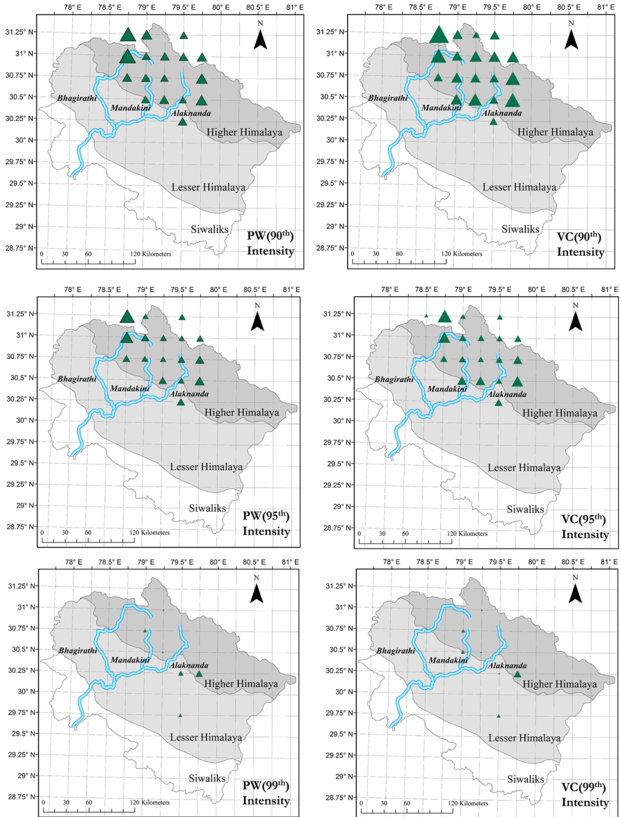
Fig. 2 Trends in rainfall intensity for depths exceeding 90th, 95th and 99th percentile thresholds. The trends are calculated using the PW (prewhitening) and VC (variance-correction) methods. Relative sizes of triangles represent relative slope magnitudes of statistically significant trends (Tables S1, S3, S5 of Supplementary shows magnitude of trends in rainfall intensity for 90th, 95th and 99th percentile thresholds, respectively)
