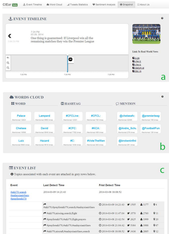
Figure 3: The Event Summarization and Event List of CLEAR System
