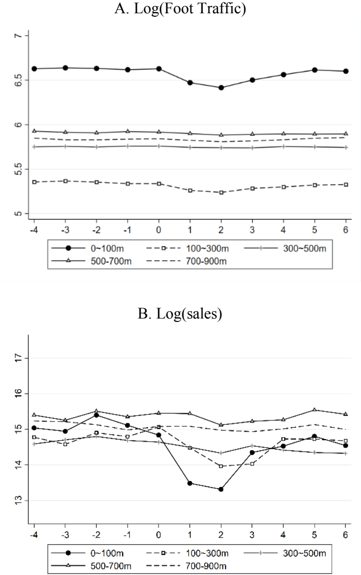
Figure A3. Trends of Foot Traffic and Sales by Distance to the Guro Call Center
