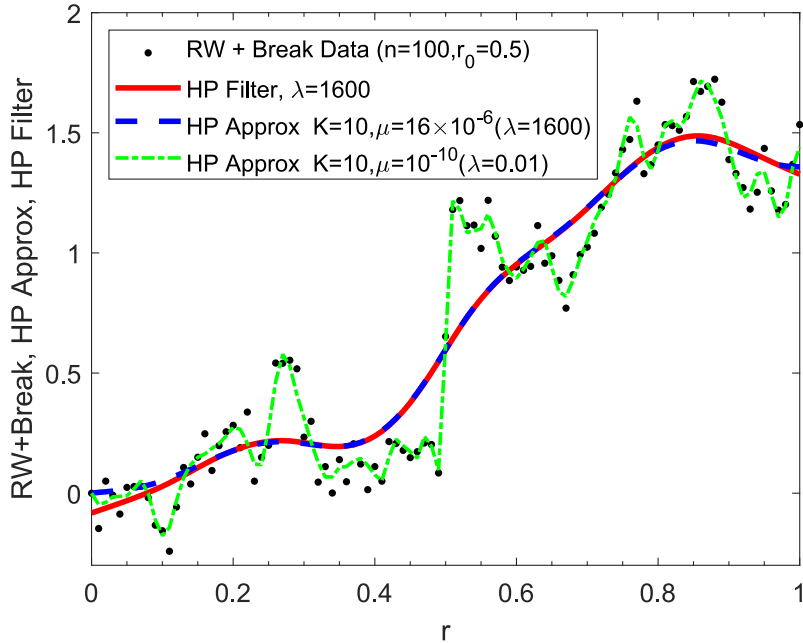
Figure 8: Random walk with a location shift at r_0 = 0.5 , shown against the HP filtered series and HP limit approximations ( \mu = 16 \times 10^{-6} and \mu = 10^{-10} ).
