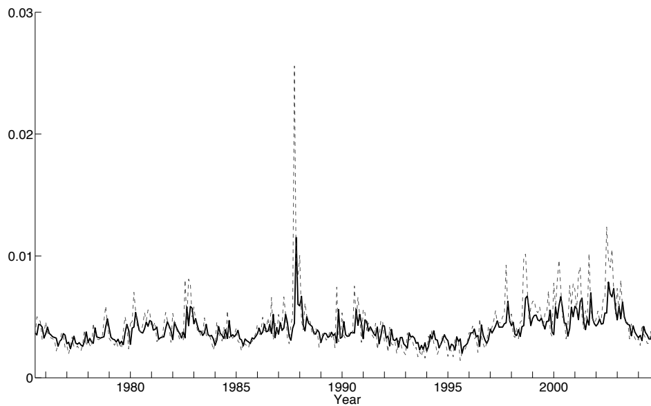
Figure 4. Realized volatility and out-of-sample TNTAR forecasts for the period Jul 1975–Dec 2004. Dashed line: S&P 500 monthly realized volatility. Solid line: one-step-ahead TNTAR forecasts.
