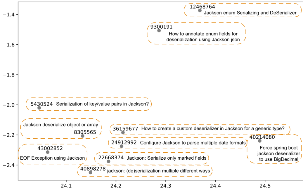
Figure 4.5: Vector Space
