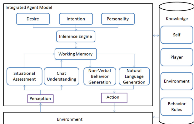
Figure 1. A schematic of the integrated agent model.
