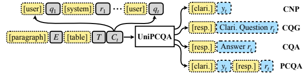
Figure 3: Overview of the input/output for UniPCQA. Note that the first three outputs denote the output in the single-task learning setting for each sub-task, while the last one denotes that in the multi-task learning setting.
