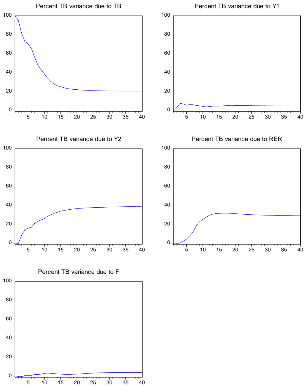
Figure 5 Variance Decomposition
