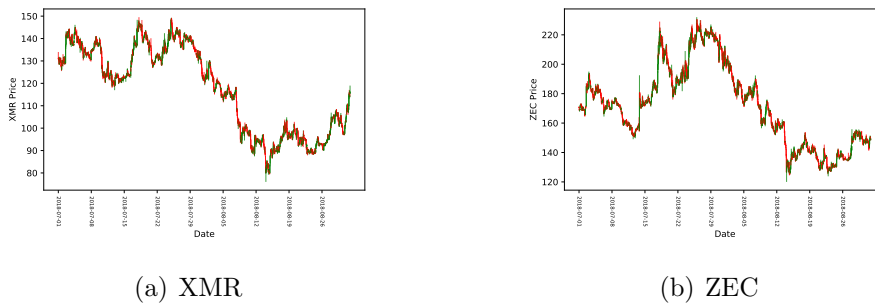
Figure 25: Chandelestick charts for individual price movements. 01. July 2018 - 31. August 2018.
