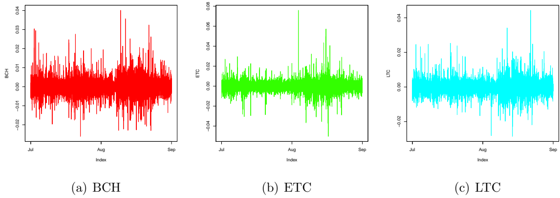
Figure 12: Intraday 5-minutes log-returns. 01. July 2018 - 31. August 2018.
