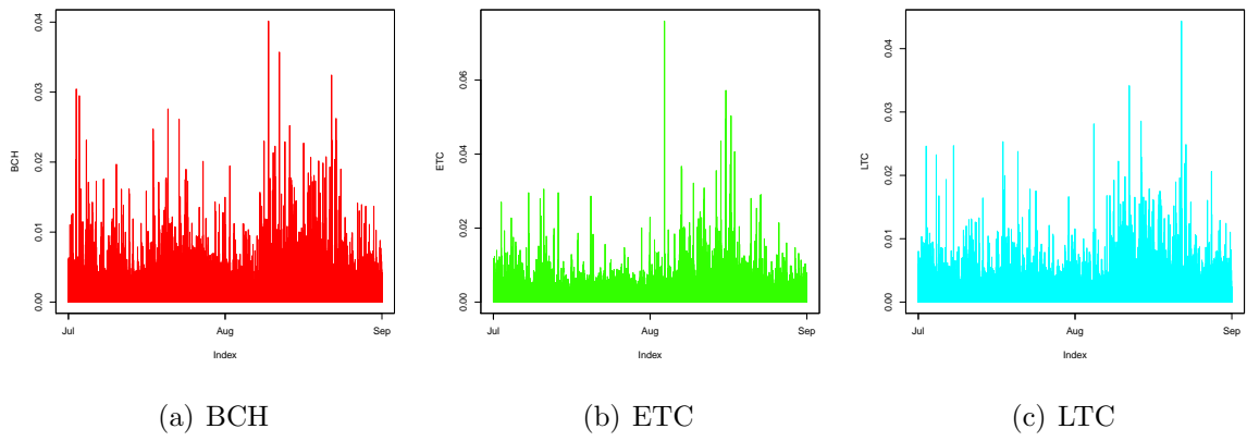
Figure 13: Intraday volatility (absolute values of 5-minutes log-returns) . 01. July 2018 - 31. August 2018.
