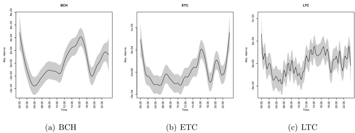
Figure 14: Generalized additive model of volatility. 01. July 2018 - 31. August 2018.
