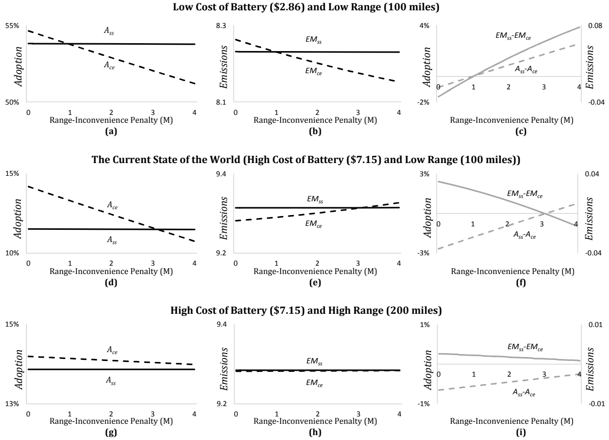
The black lines represent the conventional (dashed) and switching-station models (solid); the gray lines illustrate the differences in emissions (solid) and adoption (dashed). Emissions are in kg of CO_2 .
