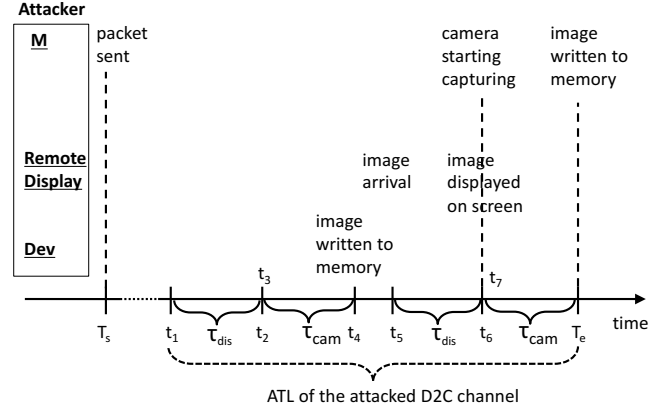
Fig. 6: Example of ATL of D2C channel under analog cuckoo attack.
