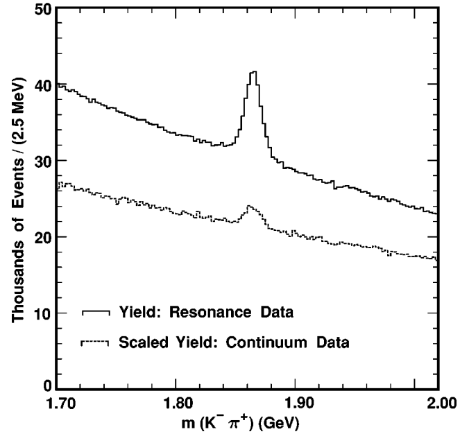
FIG. 1. The m(K^-\pi^+) distribution for D^0 candidates ( 0.0 < x_D < 0.50 ) (where x_D = p_D/p_{\max} ) from ‘‘on-resonance’’ data ( p_{\max} = 4.950 GeV/ c ) and from ‘‘continuum’’ data ( p_{\max} = 4.920 GeV/ c ). The ‘‘continuum’’ distribution is scaled by the luminosity and cross section factor 2.080.
