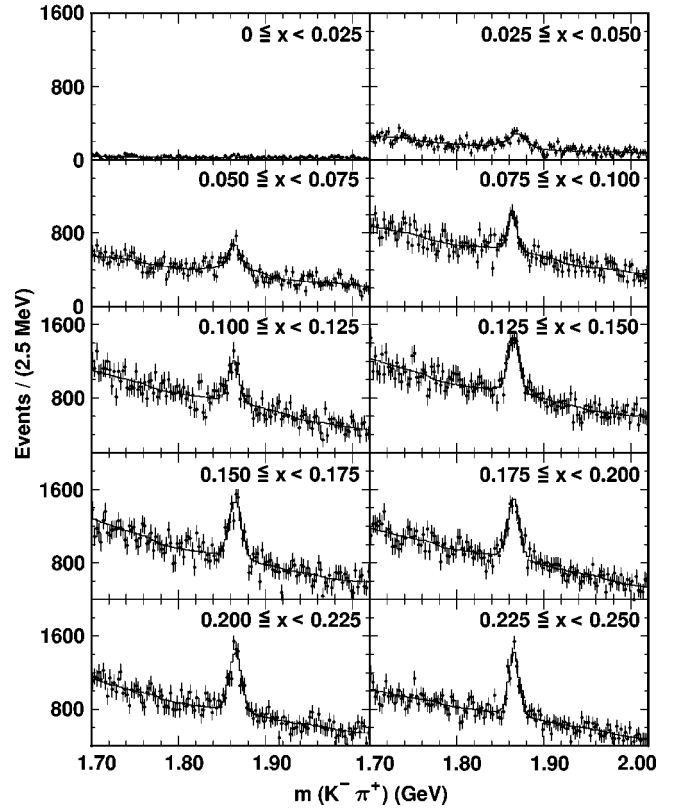
FIG. 12. The m(K^- \pi^+) distribution for B \rightarrow D^0 X candidates in ten x bins from 0 to 0.25. The histogram is the result of the fit.
