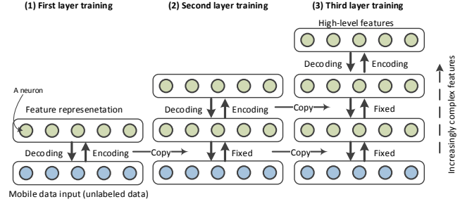
Fig. 2: Generative layer-wise training of a deep model. Each layer applies nonlinear transformation to its input vector and produces intrinsic features at its output.
