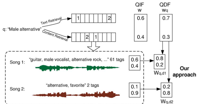
Fig. 1. A retrieval and fusion example.
