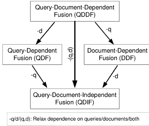
Fig. 2. Transitions between different multimodal fusion approaches.
