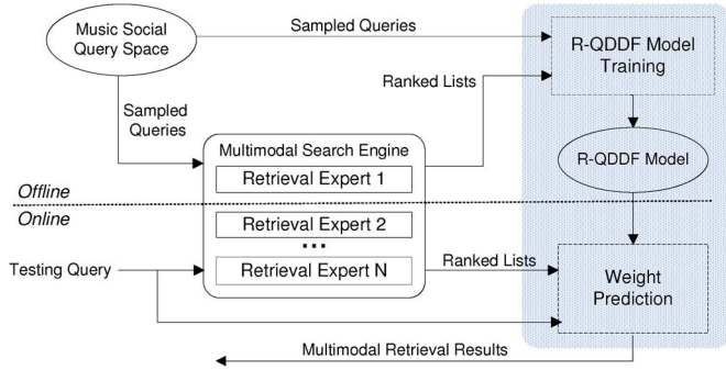
Fig. 4. Regression-based fusion weight learning diagram.
