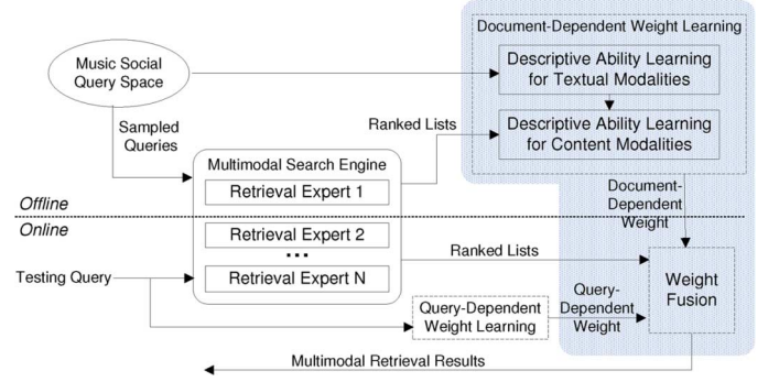
Fig. 3. Dual-phase fusion weight learning diagram.
