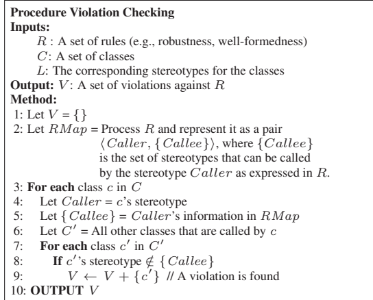
Figure 2. Violation Detection
