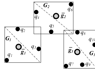
Figure 6: Service provider partitioning
