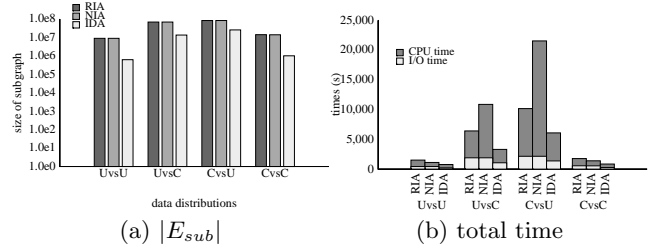
Figure 13: Different distributions (default k, |Q|, |P| )
